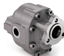
3 bolts UNI (21 UNI 222)
